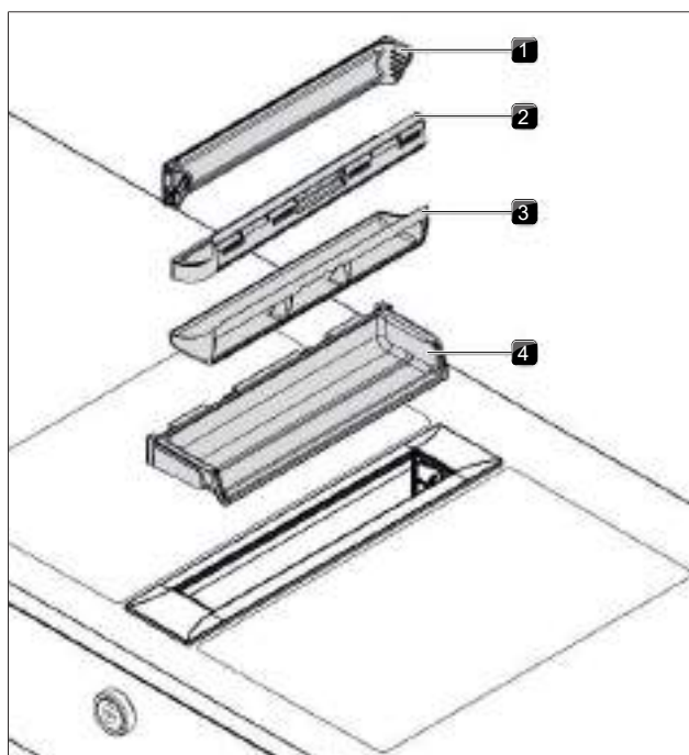
Fig. 3.7 Filter components
