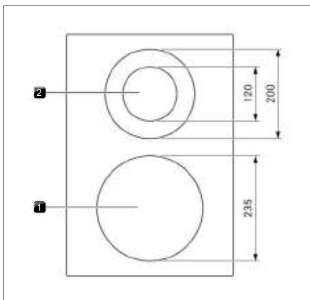
Fig. 3.13 Layout of cooktop PKCH3 and cooking zone dimensions
