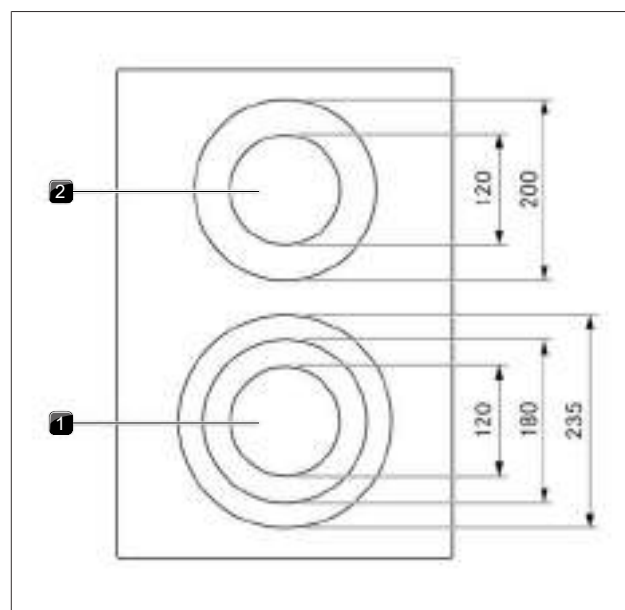
Fig. 3.11 Layout of cooktop PKC3 and cooking zone dimensions
