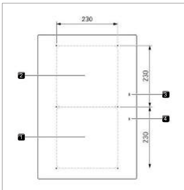
Fig. 3.8 Layout of cooktop PKFI3 / PKFI3R and size of the cooking zones
